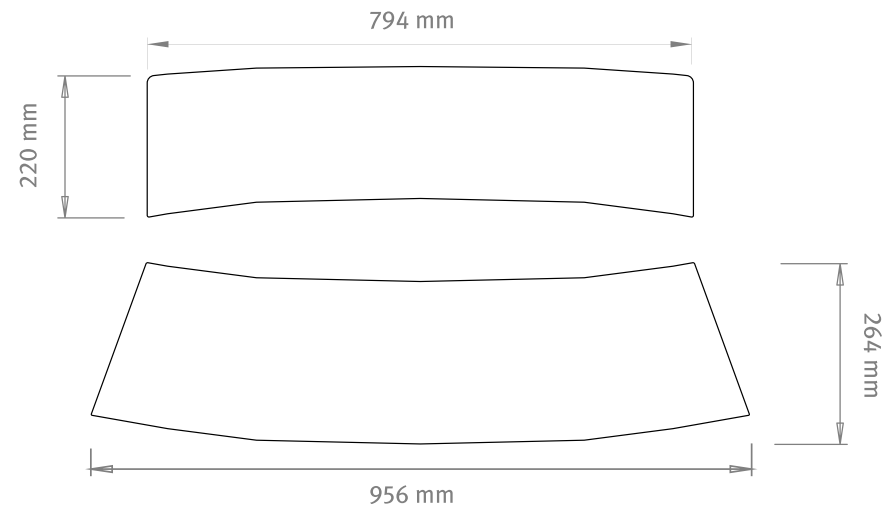
Front bottom panel Babboe Curve
