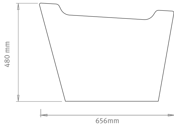
Side panel Babboe Curve (2x)
