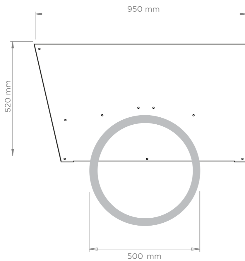
Side panel (2x)
