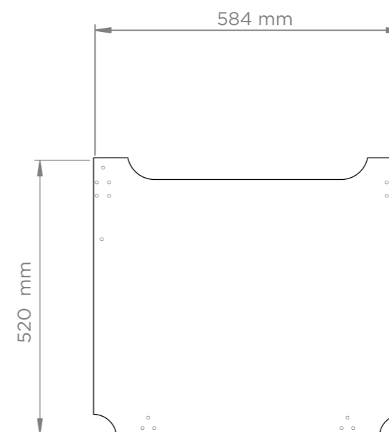
Front panel
